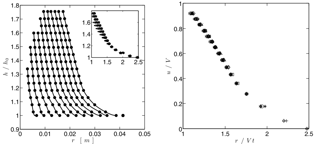
Fig. 8. Left: Thickness profiles of the aureole at successive instants of the bursting sampled every 320 \mu\text{s} . Dots represent measurements and lines are meant to guide the eyes. Inset: the same profiles plotted versus r/Vt . Right: Liquid velocity profiles of the aureole at successive instants of the bursting versus radius r scaled by the current edge position Vt sampled every 320 \mu\text{s} .
